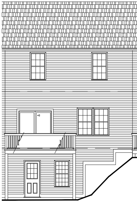
REAR ELEVATION
