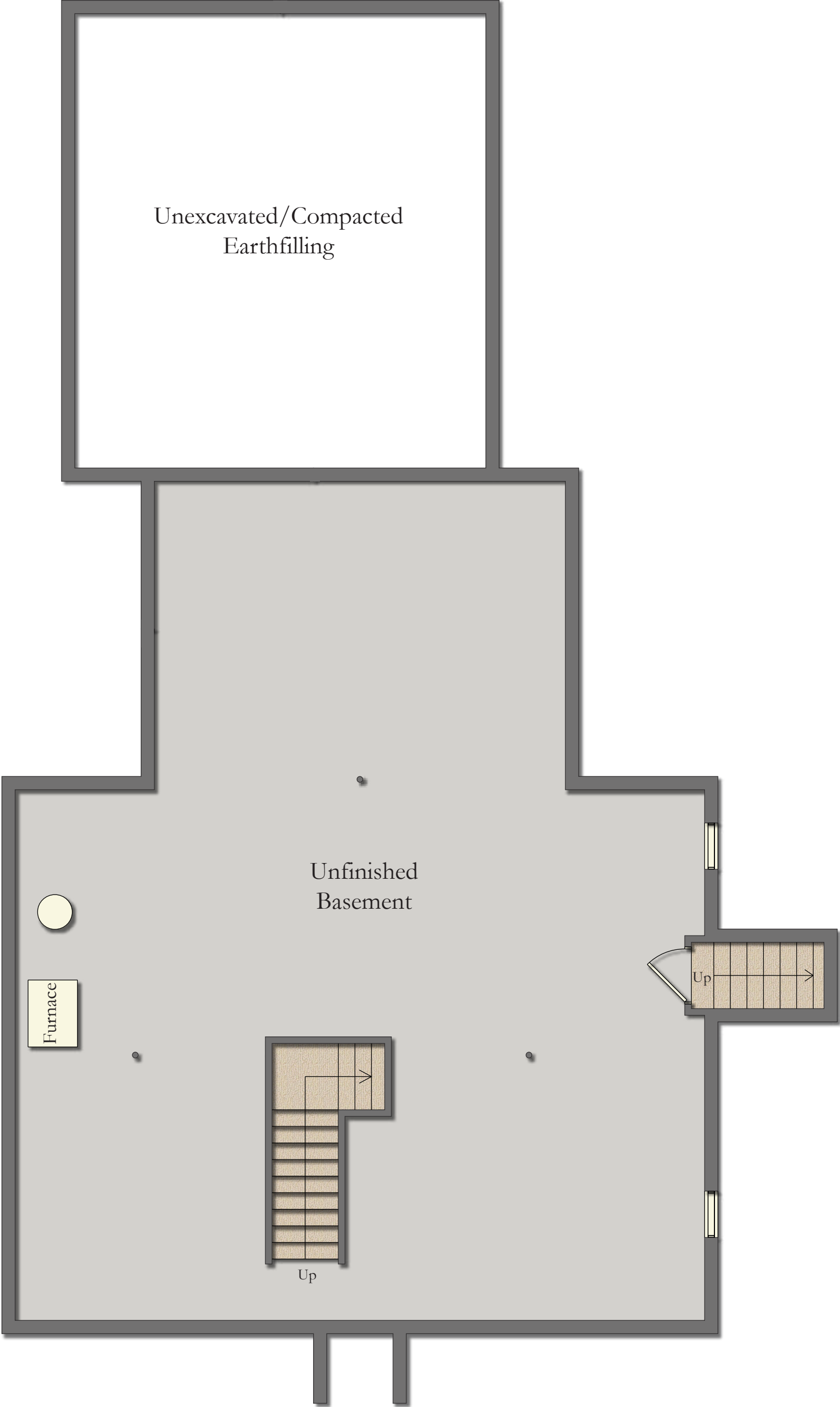
Basement Plan
